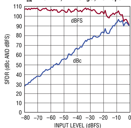
LTC2264-14: SFDR vs Input Level, f_{IN} = 70\text{MHz} , 2\text{V} Range, 40\text{Mps}
