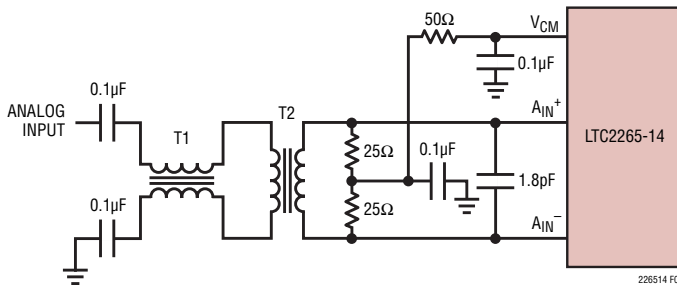
Figure 4. Recommended Front-End Circuit for Input Frequencies from 70MHz to 170MHz
